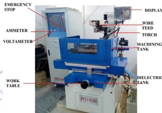
Fig.1 EX7732 CNC WEDM Machine
